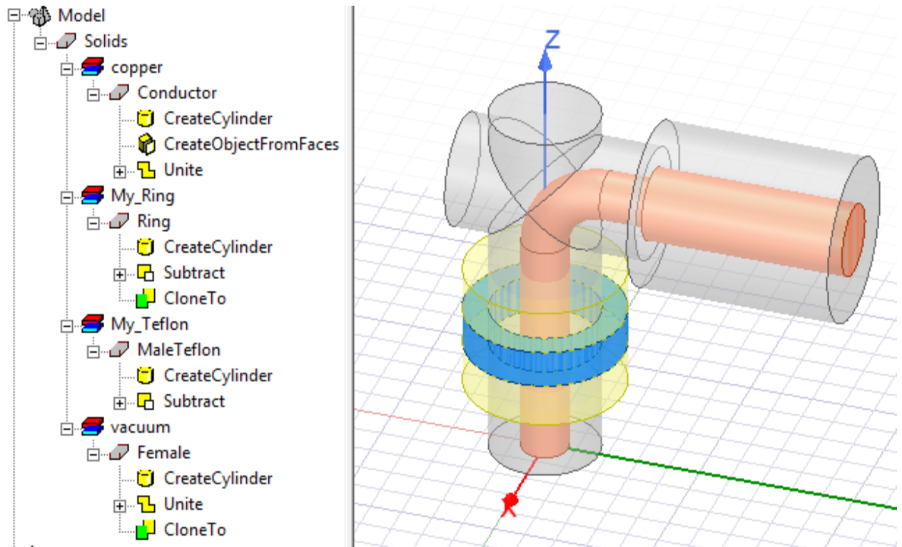
Figure 3-33: Male Teflon Created
