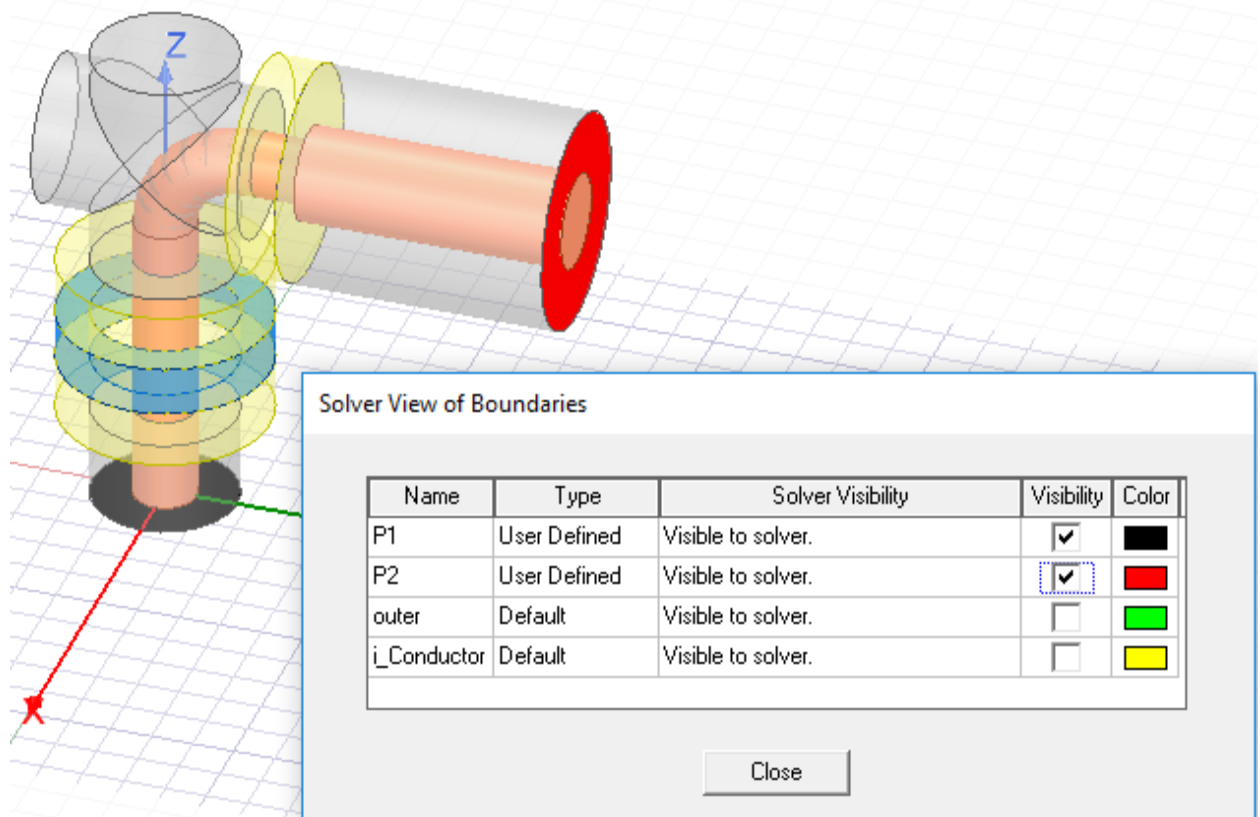
Figure 3-46: Solver View of Boundaries – P1 and P2 Boundaries Displayed
