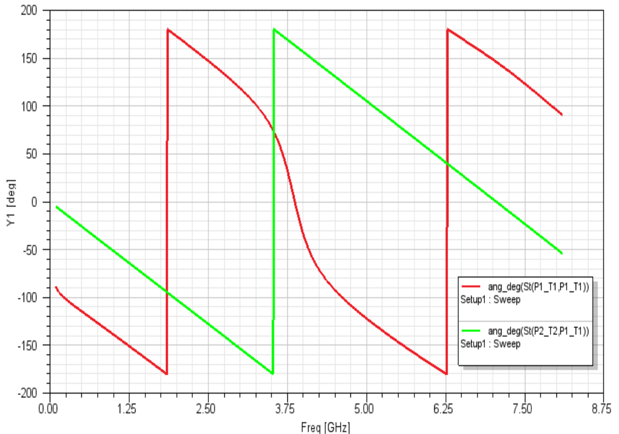
Figure 4-16: S Parameter (Angle) vs. Frequency Plot
